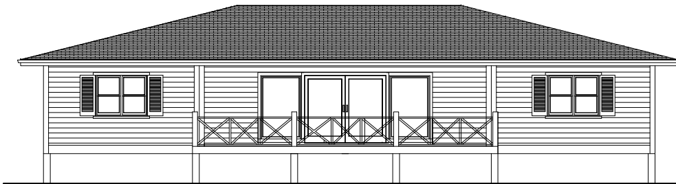
REAR ELEVATION
