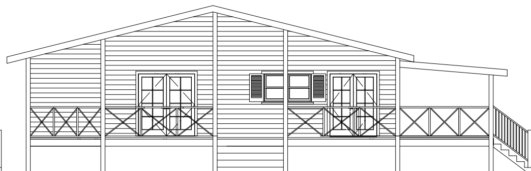
SIDE ELEVATION
