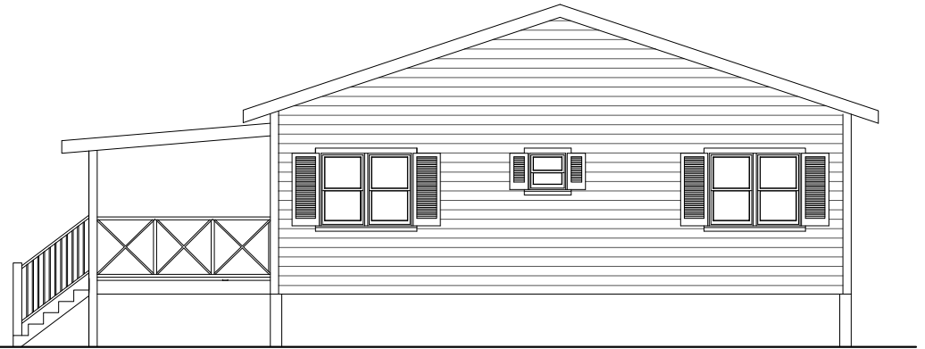
SIDE ELEVATION
