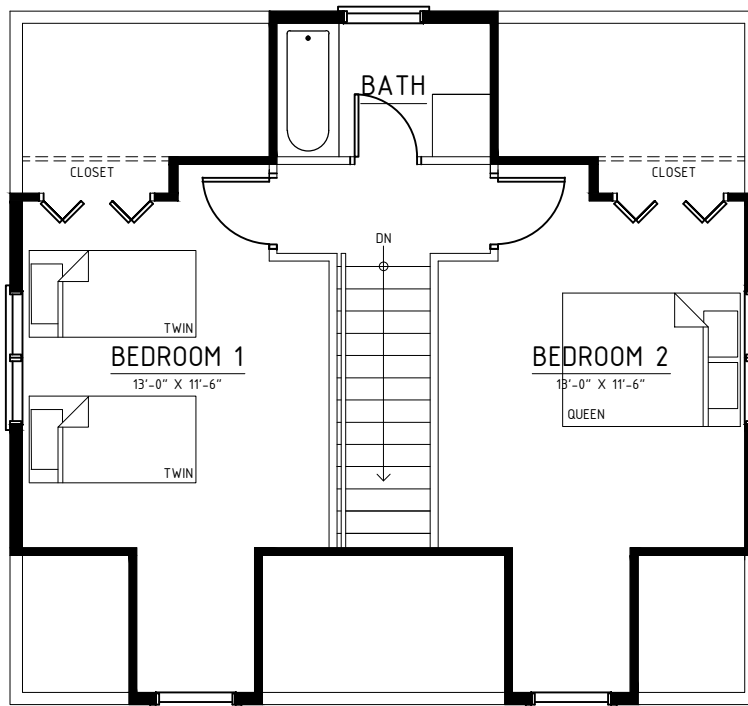
LOFT FLOOR PLAN
